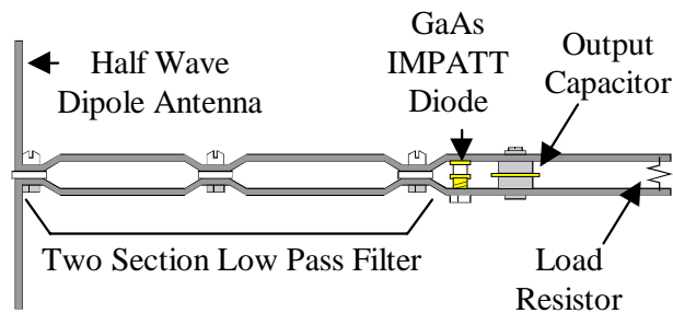
Fig 2. Rectenna element configuration.
