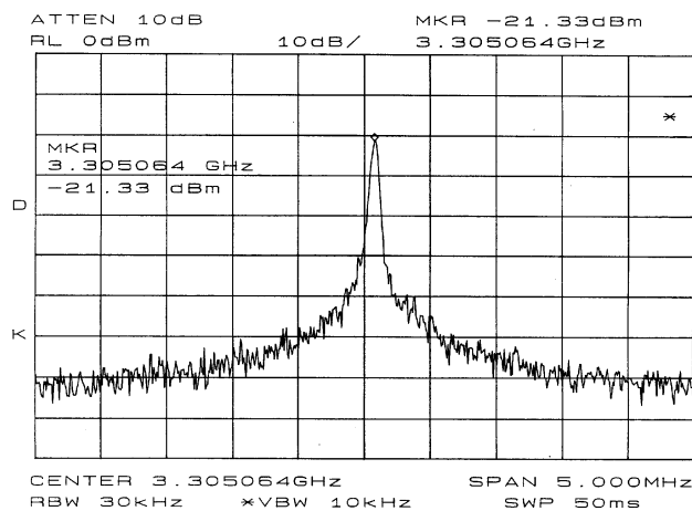
Fig 4. Measured spectrum of the oscillating rectenna.
