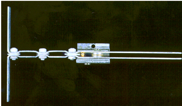
Fig 1. Photograph of rectenna element.
