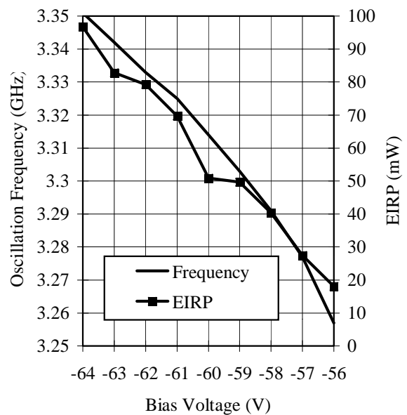
Fig 3. Oscillation frequency and EIRP vs. IMPATT bias voltage.
